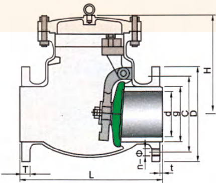
主要外形尺寸和连接尺寸 (mm) Main External and Connecting Dimensions(mm)
